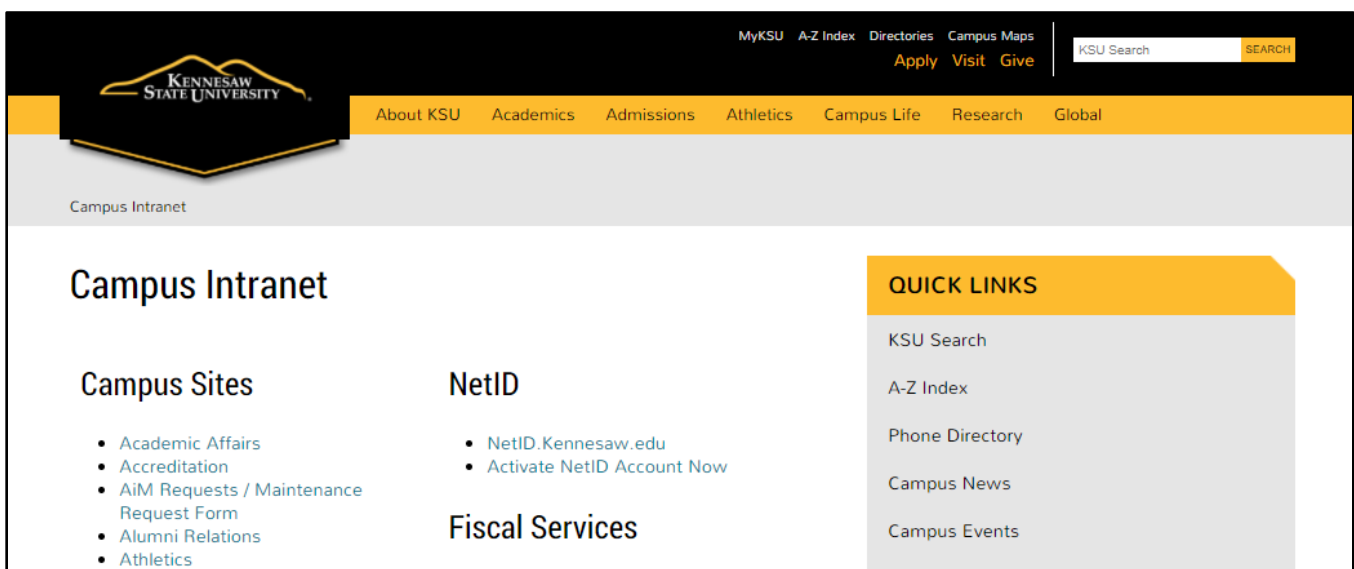
Figure 10 - Campus Intranet
