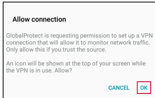
Figure 9 - Allow Connection
