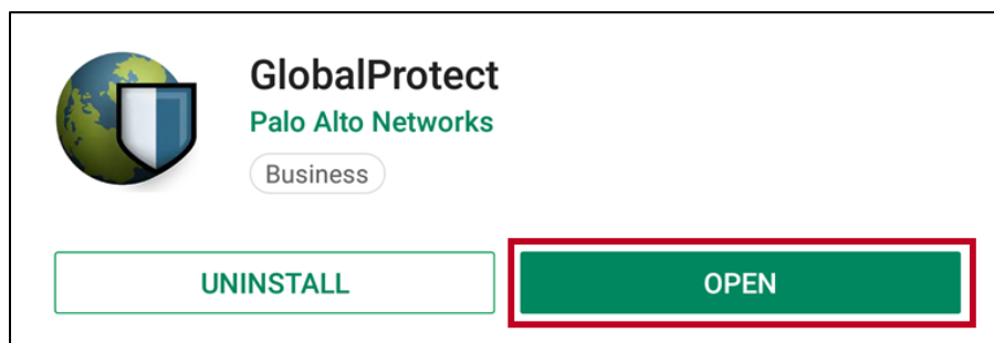
Figure 5 - Open GlobalProtect
