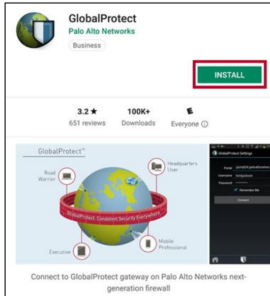
Figure 3 - GlobalProtect App
