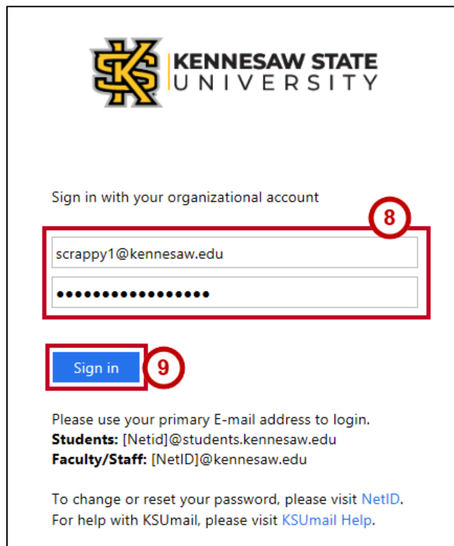
Figure 7 - Sign In
