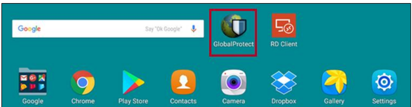
Figure 11 - GlobalProtect App
