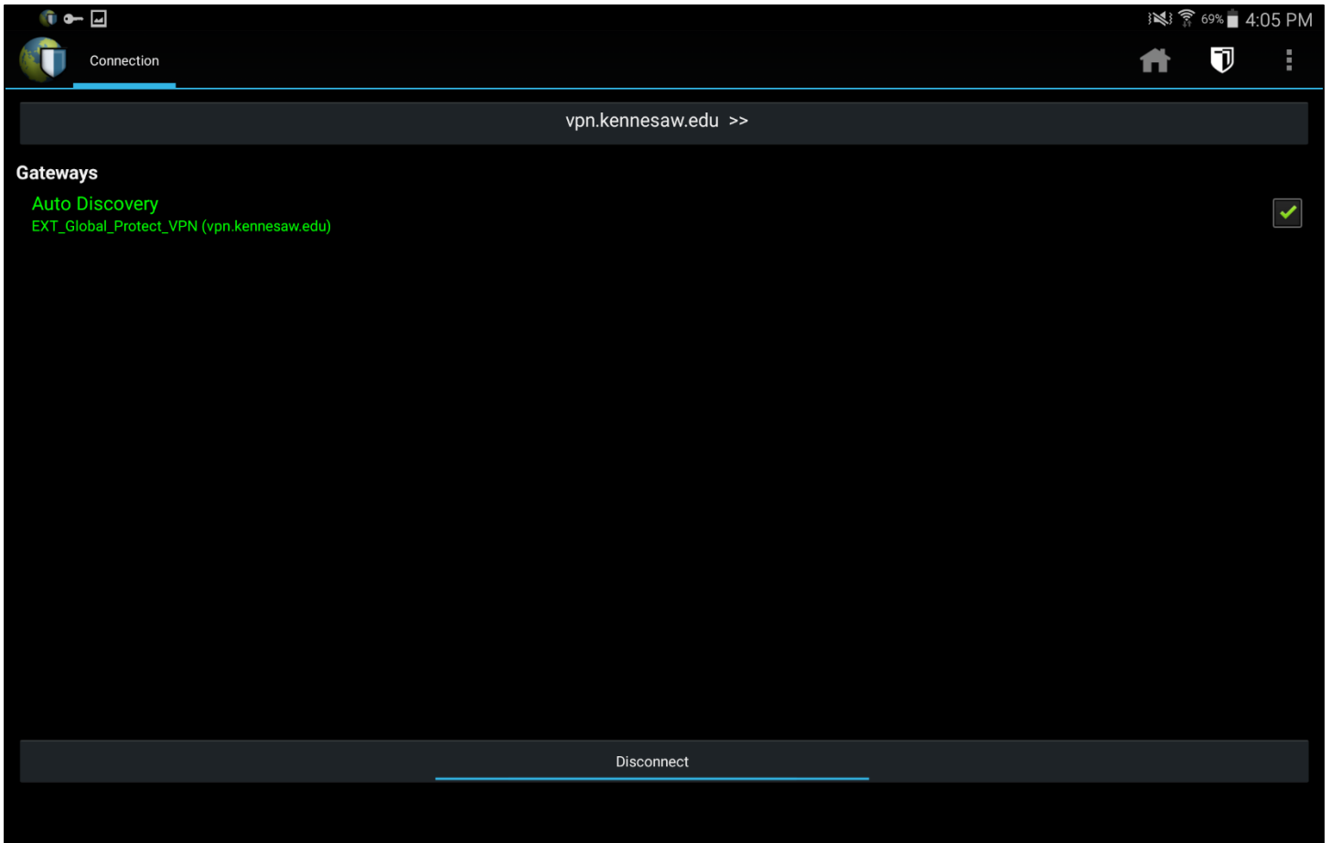
Figure 12 - Disconnect
