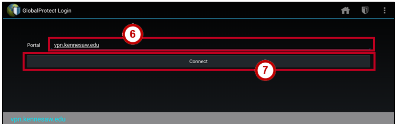
Figure 6 - GlobalProtect Portal
