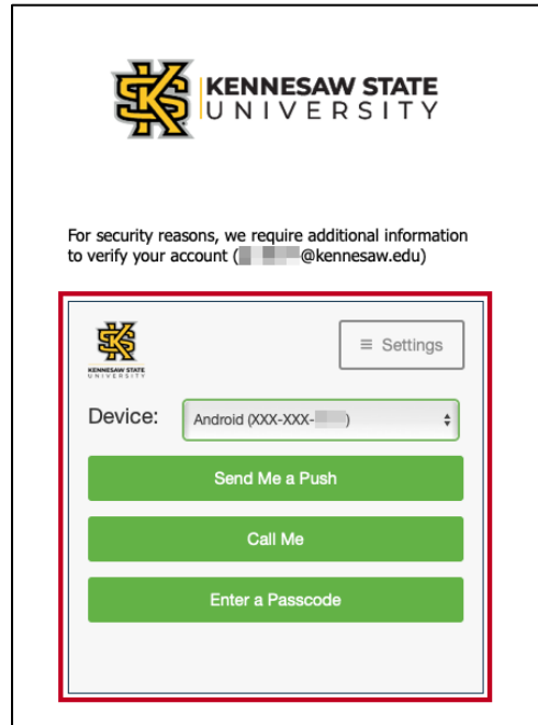
Figure 8 - Duo Verification
