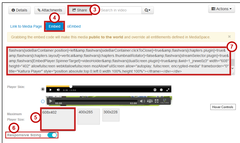
Figure 11 - Grabbing Embed Code from MediaSpace
