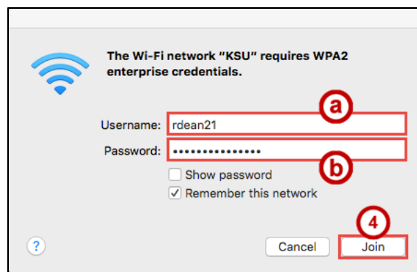
Figure 2 - Join
